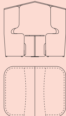
4-seater composition with table L 220 P 160 H 205 cm
