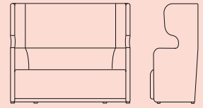
High back 2-seater sofa L 157 P 76 H 133 cm
