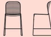
Stool L 57 P 58 H 105 cm
